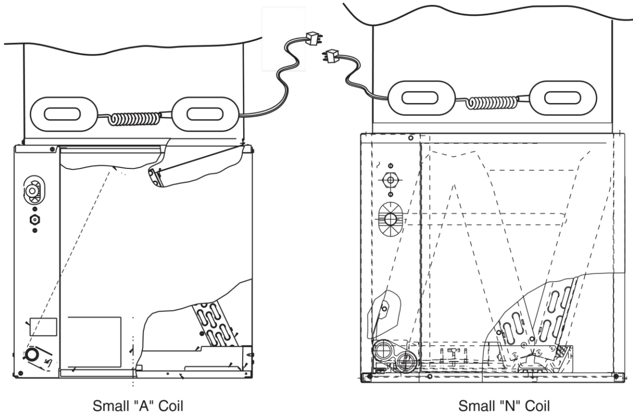
Fig. 3B—Alternate Furnace Coil Mounting Locations--115-v Application
