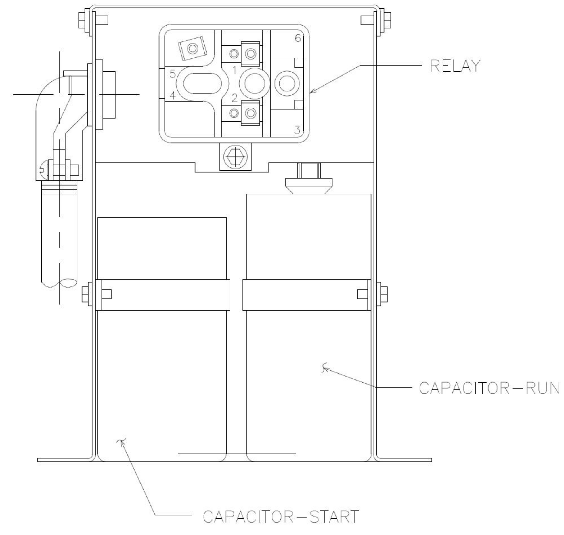
514-2000 SERIES CAPACITOR AND RELAY ASSEMBLY OFFERED ON -945 MODELS
