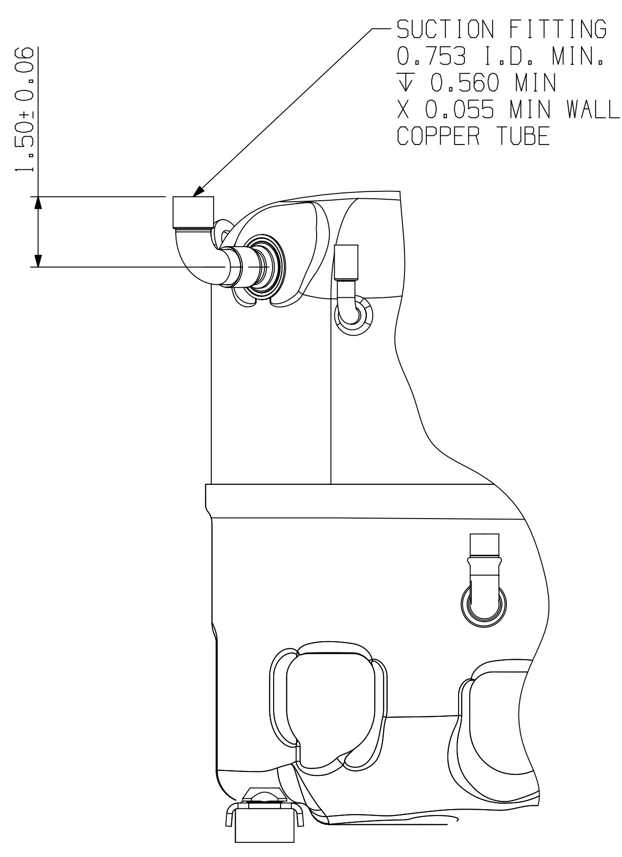
OPTION SHOWN: 0.75 ID ELBOW-UP SUCTION 0.50 ID X 0.63 OD ELBOW-UP DISCHARGE (STANDARD)
