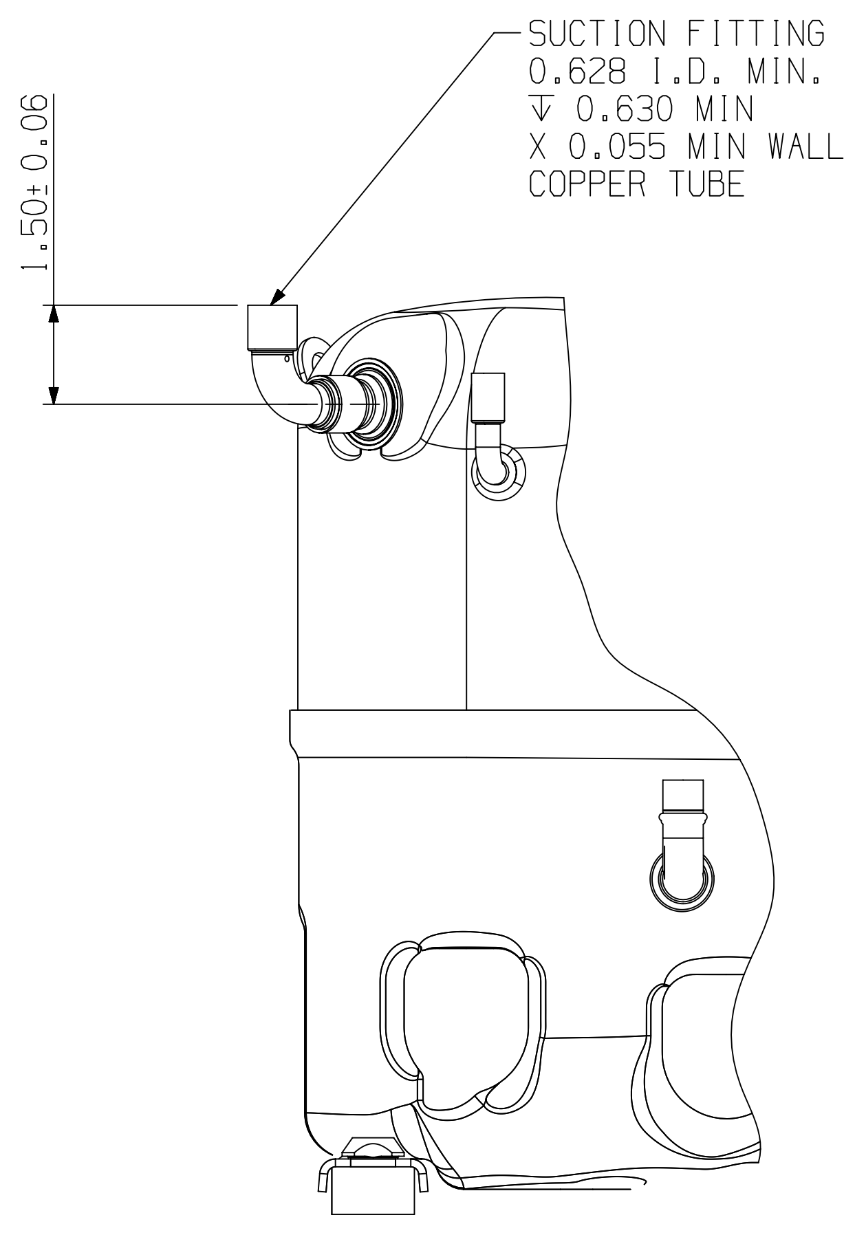
OPTION SHOWN: 0.63 ID ELBOW-UP SUCTION 0.50 ID X 0.63 OD ELBOW-UP DISCHARGE (STANDARD)
