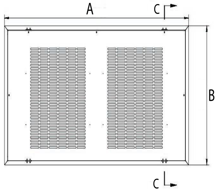
Fig. 2 – 30K/36k Louvered Panel Dimensions
