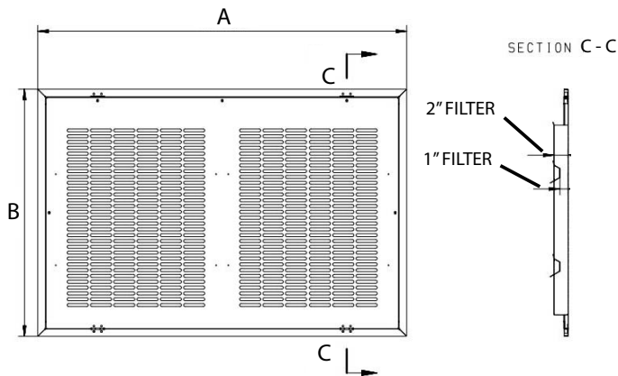
Fig. 1 – 18K/24K Louvered Panel Dimensions
