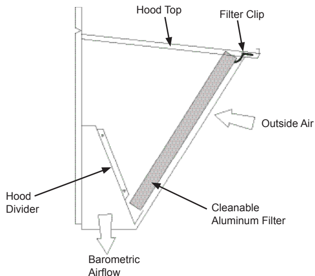
Fig. 5 - Filter Installation
