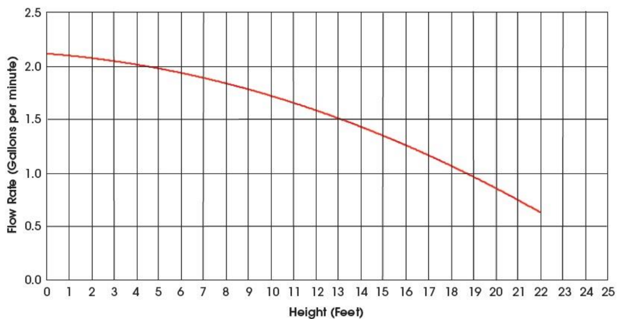
ULTRACP-22 Pump Performance Curve
