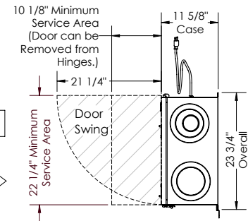
RIGHT VIEW
