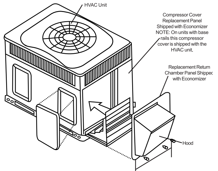
Vertical Economizer
