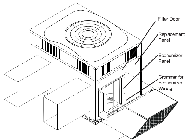
Horizontal Economizer
