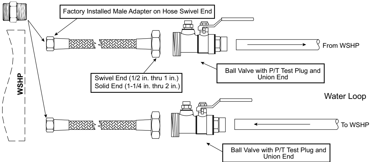
Fig. 4 — AHA**** 3/4 in. to 1-1/2 in. Stainless Steel Braided Hose Kit with Ball Valves
