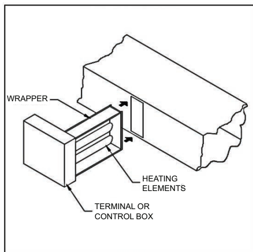
Fig. 10 — Slip-In Heater
