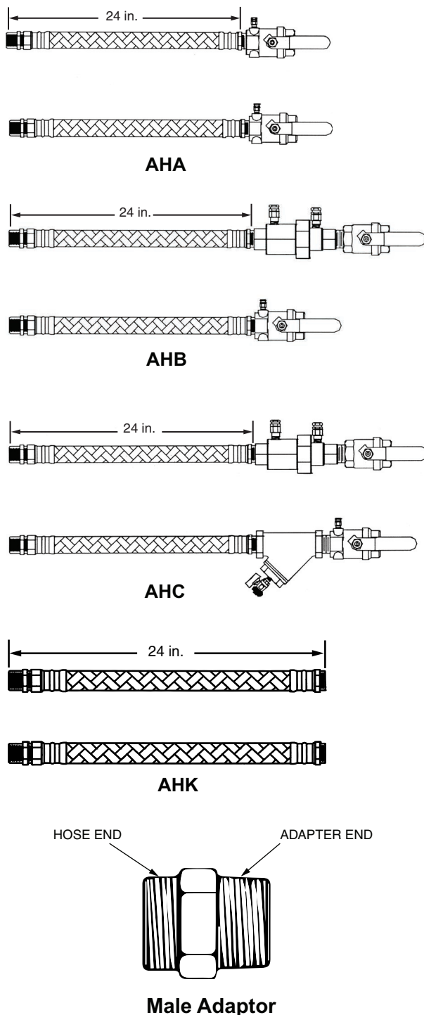
Fig. 1 — Aquazone Hose Kits
