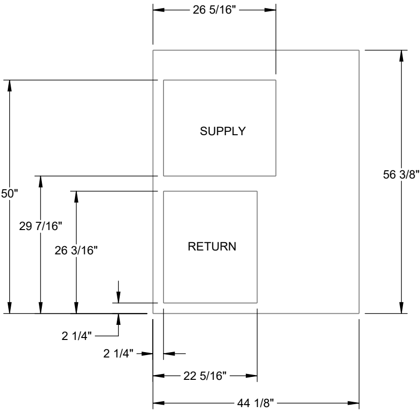
EXISTING CURB LAYOUT
