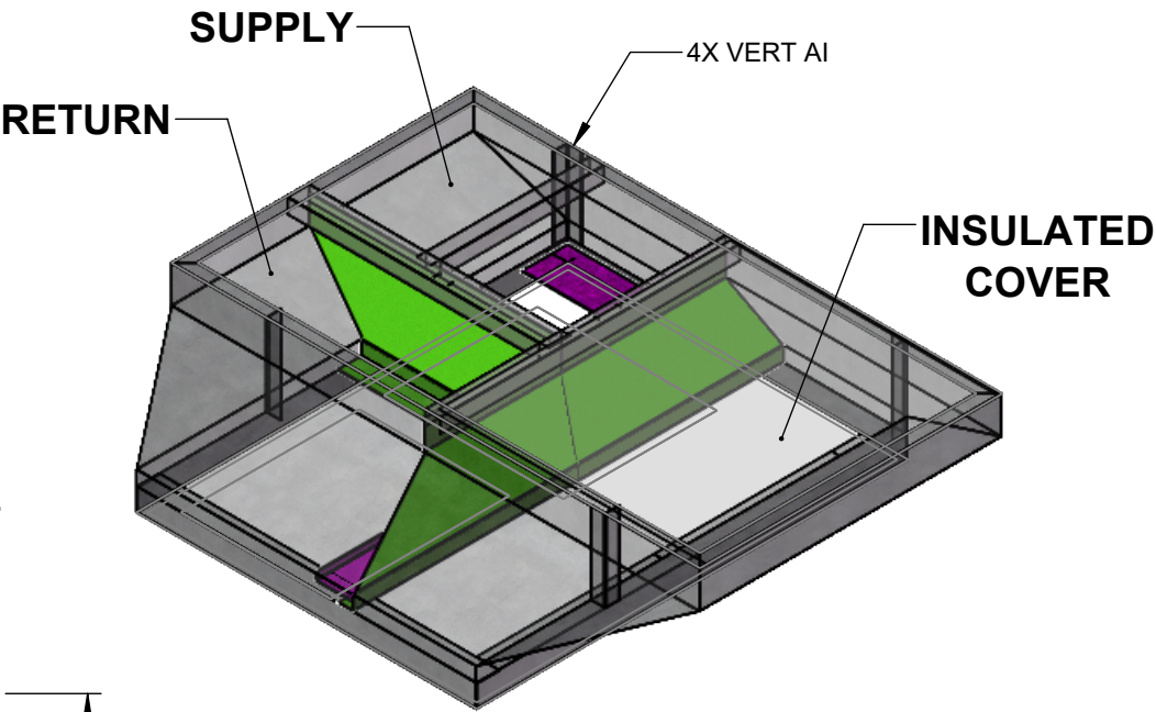
EXISTING CURB LAYOUT
