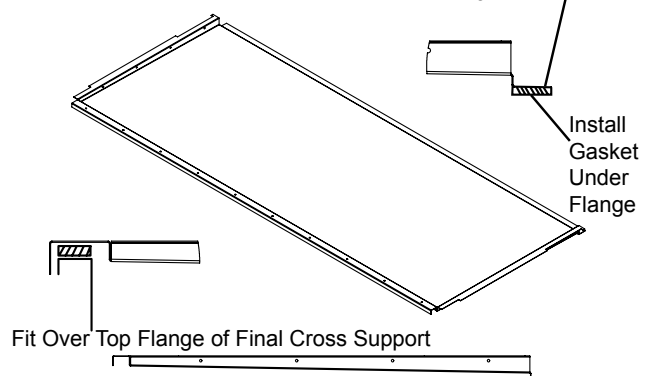
Illustration - Step 6 Sloped Deck Pans Installation
