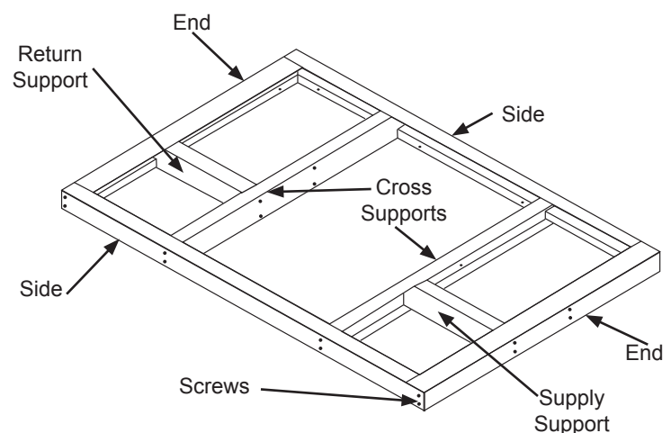
Fig. 1 - Roofcurb Adaptor
