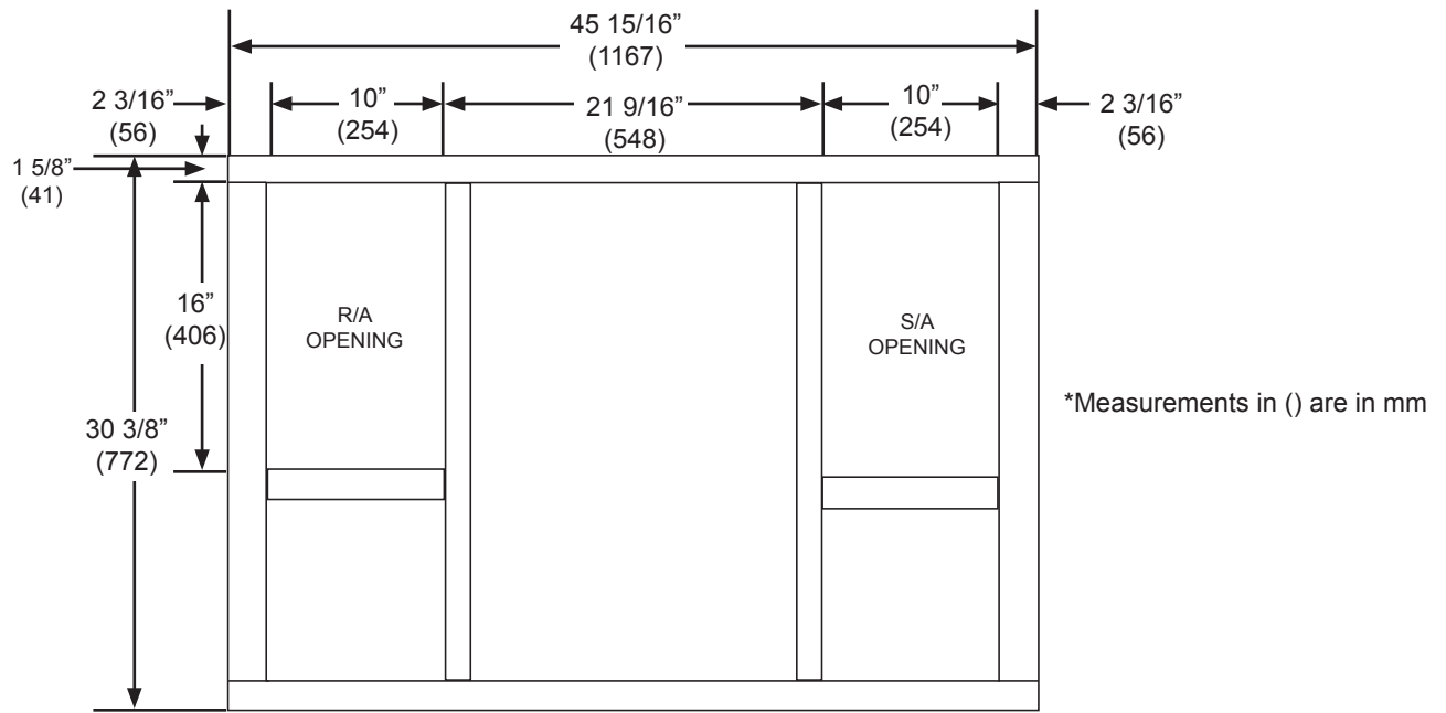
Fig. 2 - Top View
