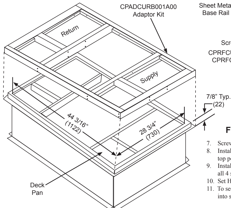
Fig. 4 - Adaptor on Existing Curb
