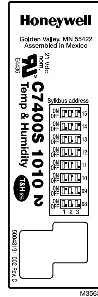
Fig. 5. Label for C7400S1010, for use on Spyder controllers.
