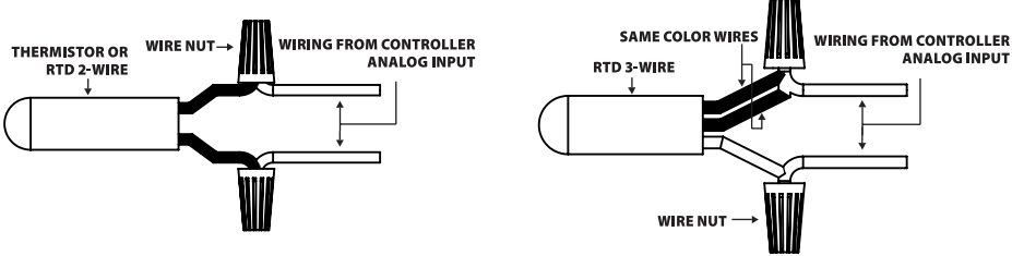
FIGURE 6: TEMPERATURE WIRING
