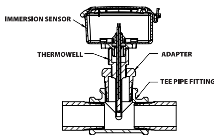
FIGURE 5: PROBE and IMMERSION
