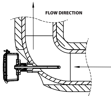
FIGURE 3: ELBOW ASSEMBLY
