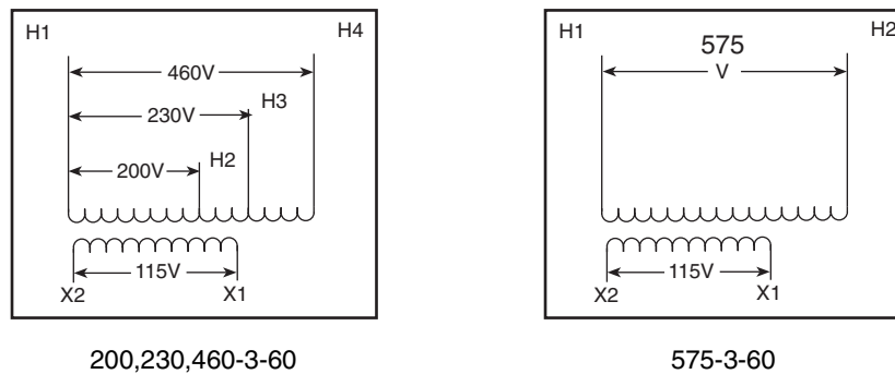
Fig. 12 — Electrical Connection Diagrams for 30HX Accessory Control Transformer
