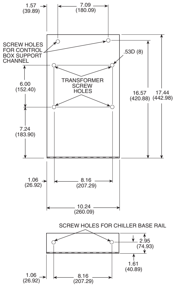
Fig. 7 — Sheet Metal Bracket for 30GXN,R Accessory Control Transformer Kits
