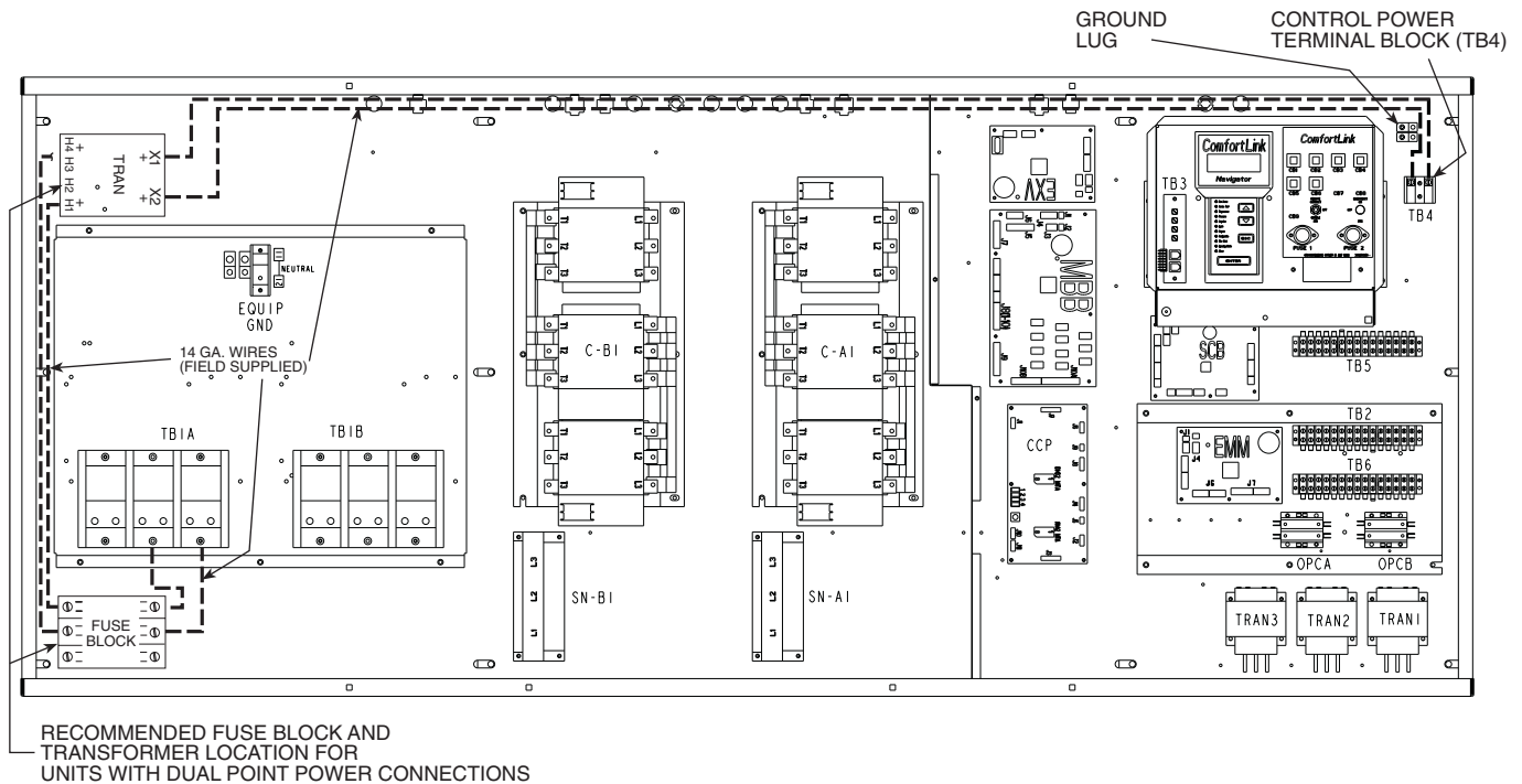
Fig. 10 — 30HX Chiller Control Panel Dual Point Power Connections (Interior, Sizes 076-186 Shown)
