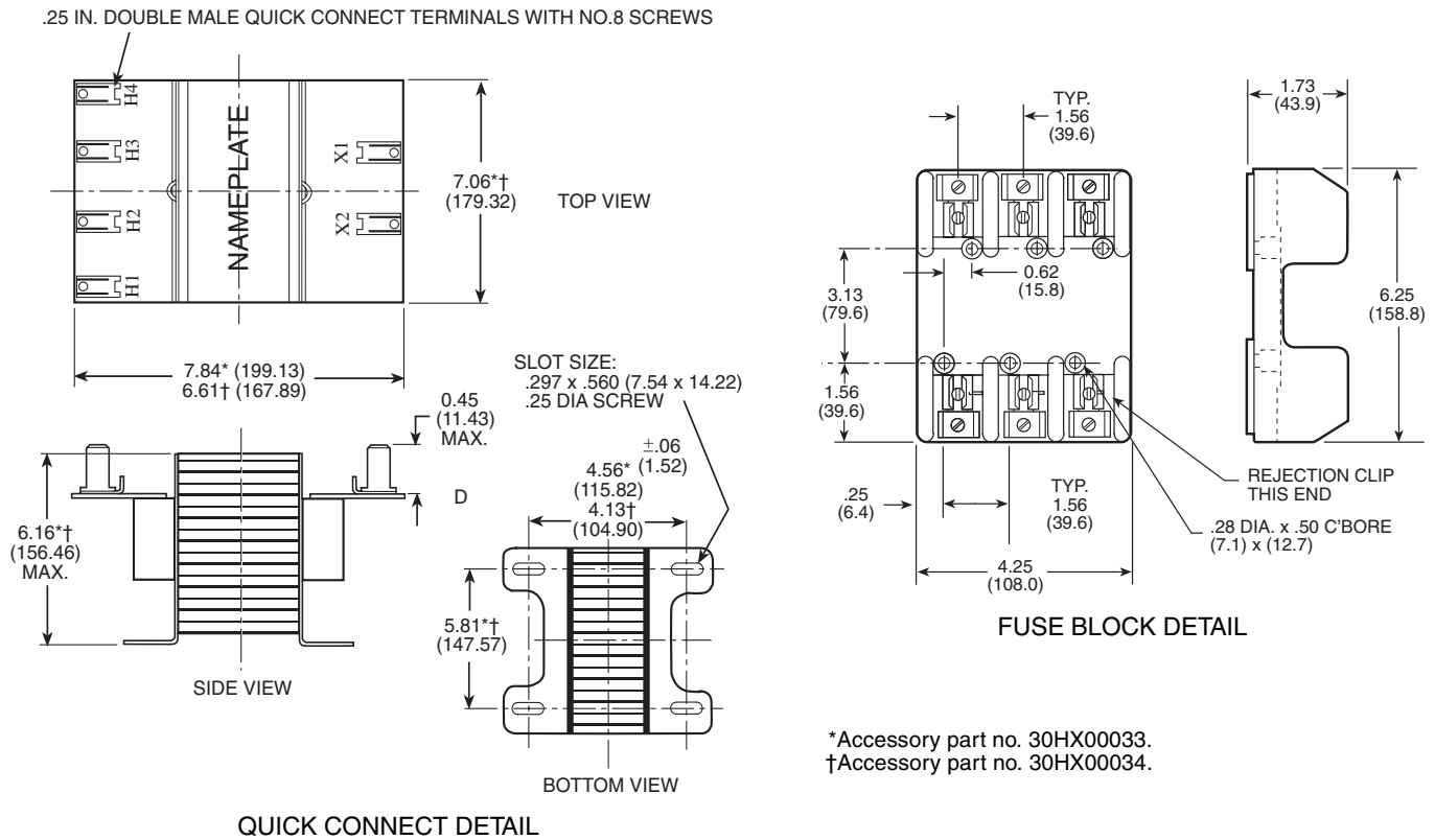
Fig. 11 — Accessory Control Transformer for Chiller Models 30HX076-271
