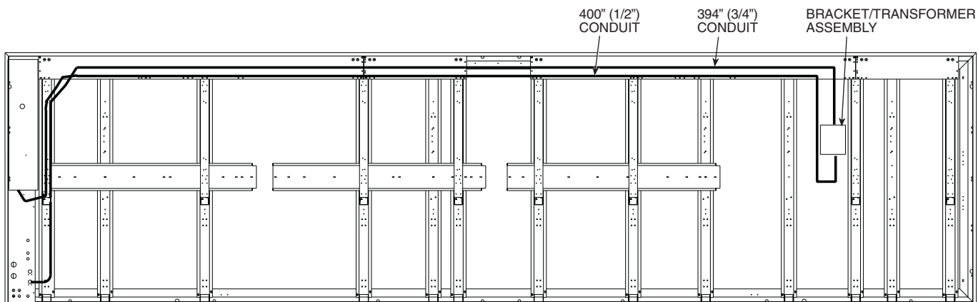
Fig. 5 — Transformer Mounting Location — 30GXN,R281-350 and Associated Modular Units
