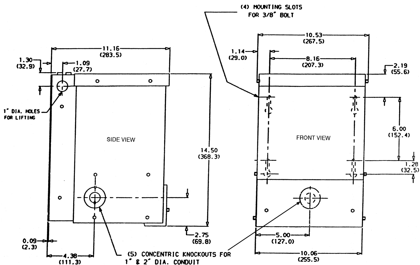
Fig. 6 — Accessory Control Transformer for Chiller Models 30GXN,R080-350
