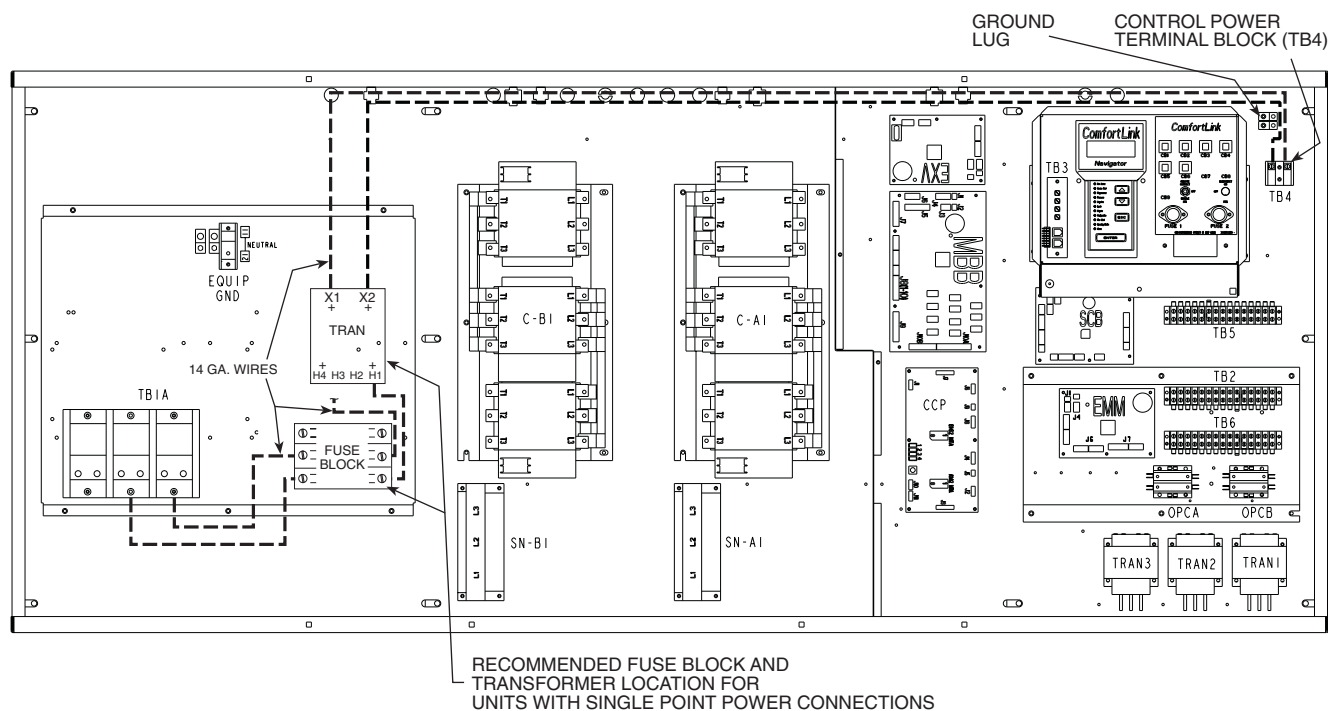
Fig. 9 — 30HX Chiller Control Panel Single Point Power Connection (Interior, Sizes 076-186 Shown)
