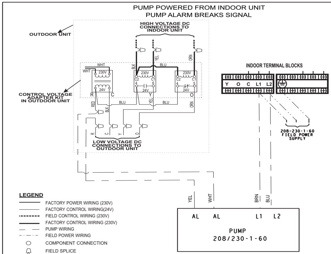
Fig. 24 – 208/230-1-60 Pump in a 208-230-1-60 40MK*B high wall HP unit -WIRING SCHEMATIC
