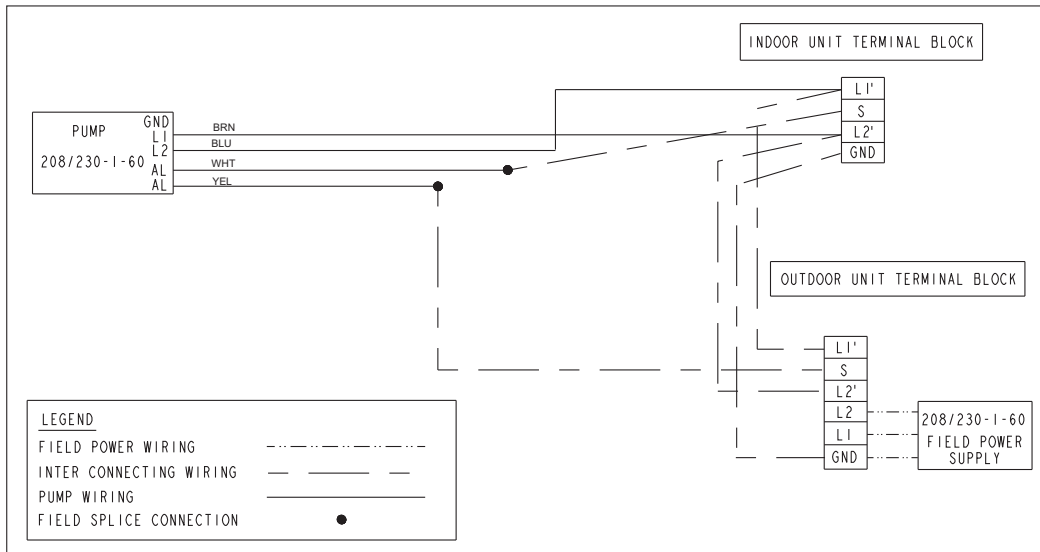
Fig. 30 – Size 18 (208-230-1-60) 40GRQ/619FB High Wall HP Unit - WIRING SCHEMATIC
