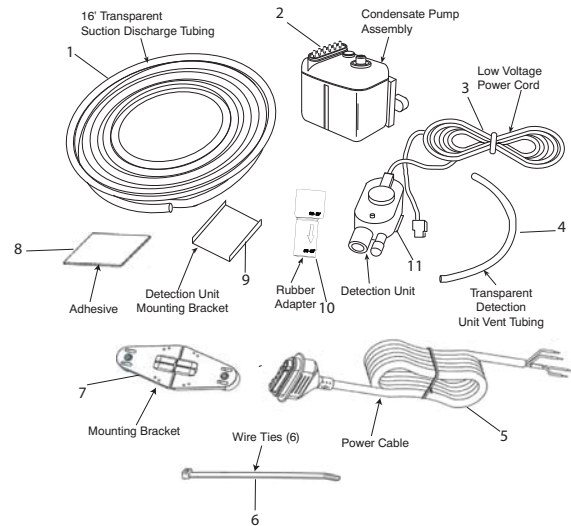
Fig. 1 – Accessory Condensate Pump Kit
