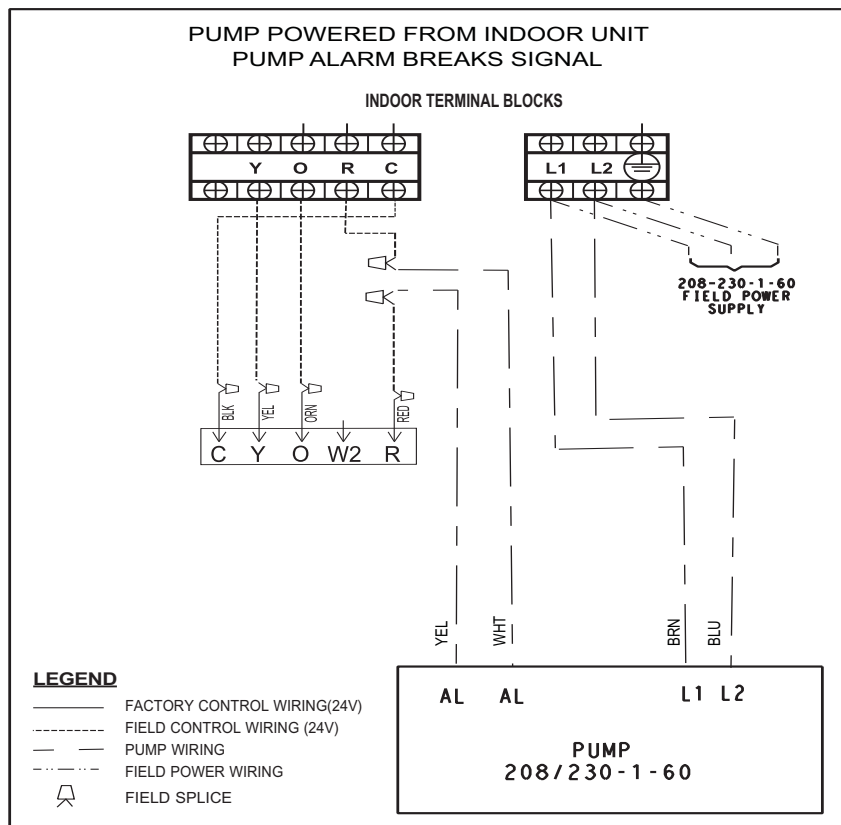
Fig. 28 – 208/230-1-60 Pump in a 208-230-1-60 40MK*F Under Ceiling HP unit - WIRING SCHEMATIC
