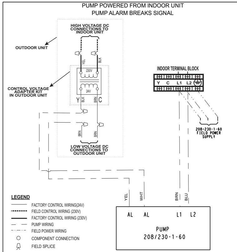
Fig. 22 – 208/230-1-60 Pump in a 208-230-1-60 40MK*B high wall AC unit - WIRING SCHEMATIC
