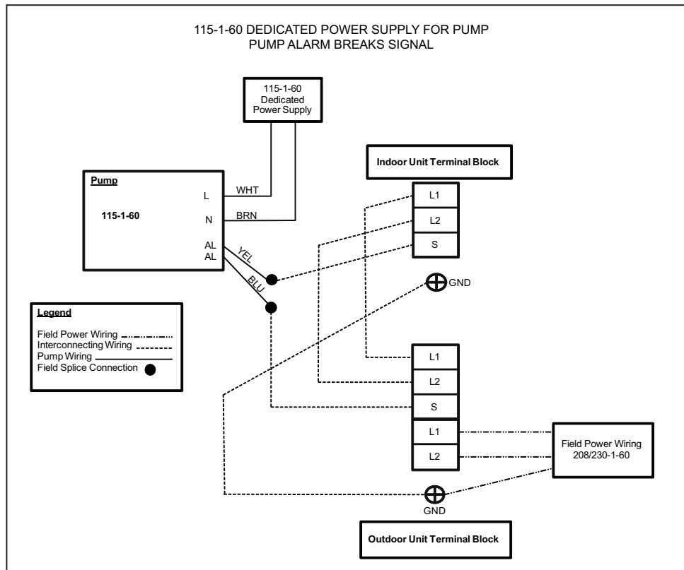
Fig. 14 – Installing a 115-1-60 Pump in a 208/230-1-60 unit-WIRING SCHEMATIC
