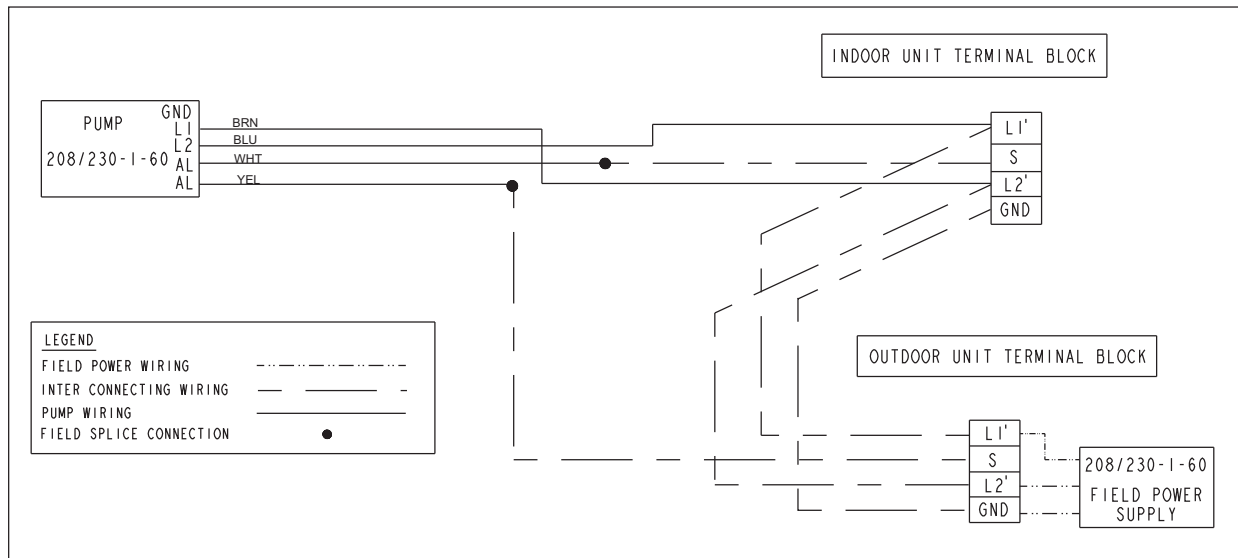
Fig. 29 – Sizes 09&12 (208-230-1-60) 40GRQ / 619FB High Wall HP Unit - WIRING SCHEMATIC
