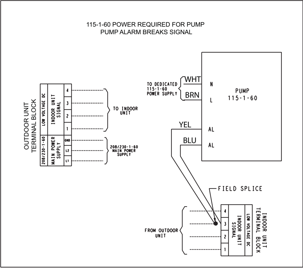
Fig. 9 – Installing a 115-1-60 Pump in a 208/230-1-60 unit-WIRING SCHEMATIC
