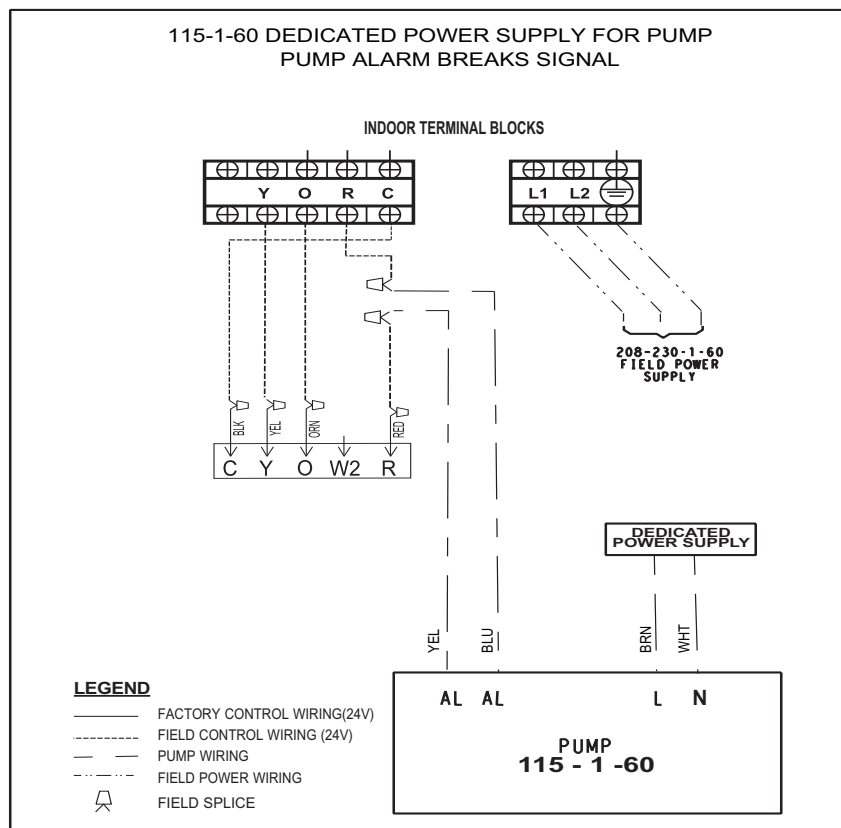
Fig. 27 – Installing a 115-1-60 in a 208-230-1-60 40MK*F Under Ceiling HP Unit - WIRING SCHEMATIC
