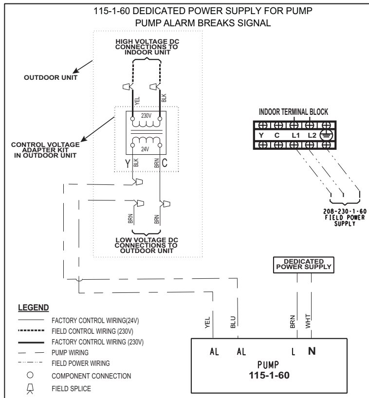
Fig. 21 – Installing a 115-1-60 Pump in a 208-230-1-60 40MK*B high wall AC unit -WIRING SCHEMATIC
