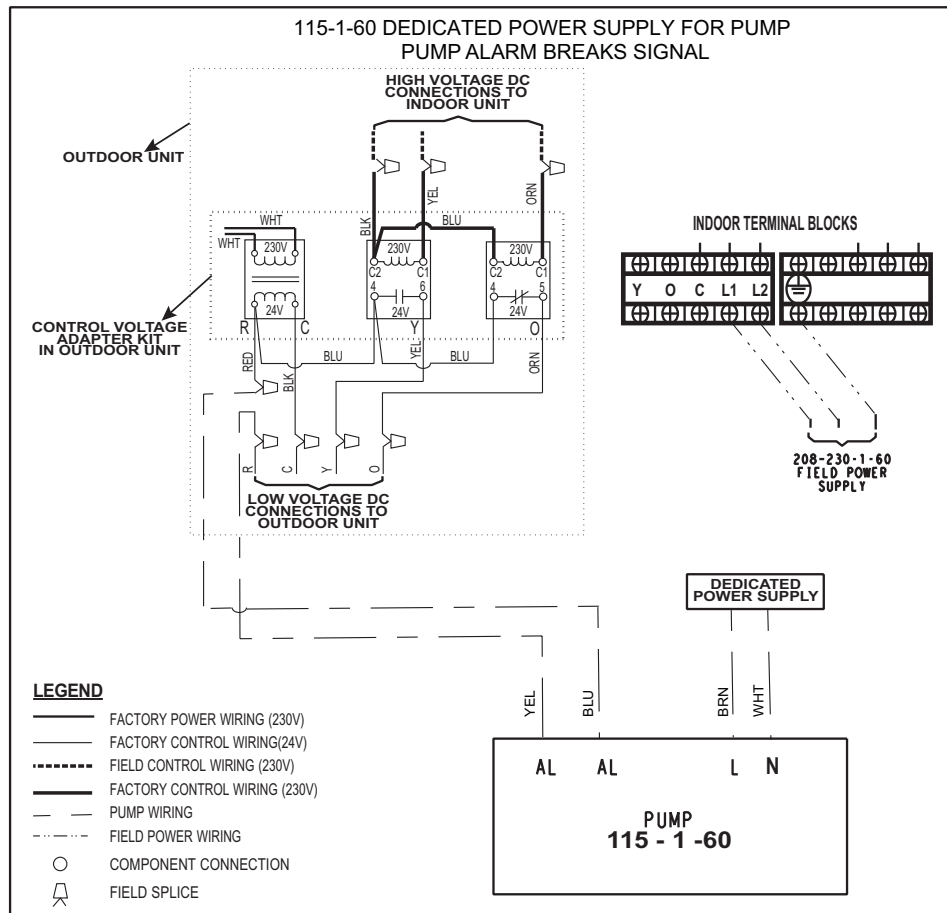
Fig. 23 – Installing a 115-1-60 Pump in a 208-230-1-60 40MK*B high wall HP unit -WIRING SCHEMATIC
