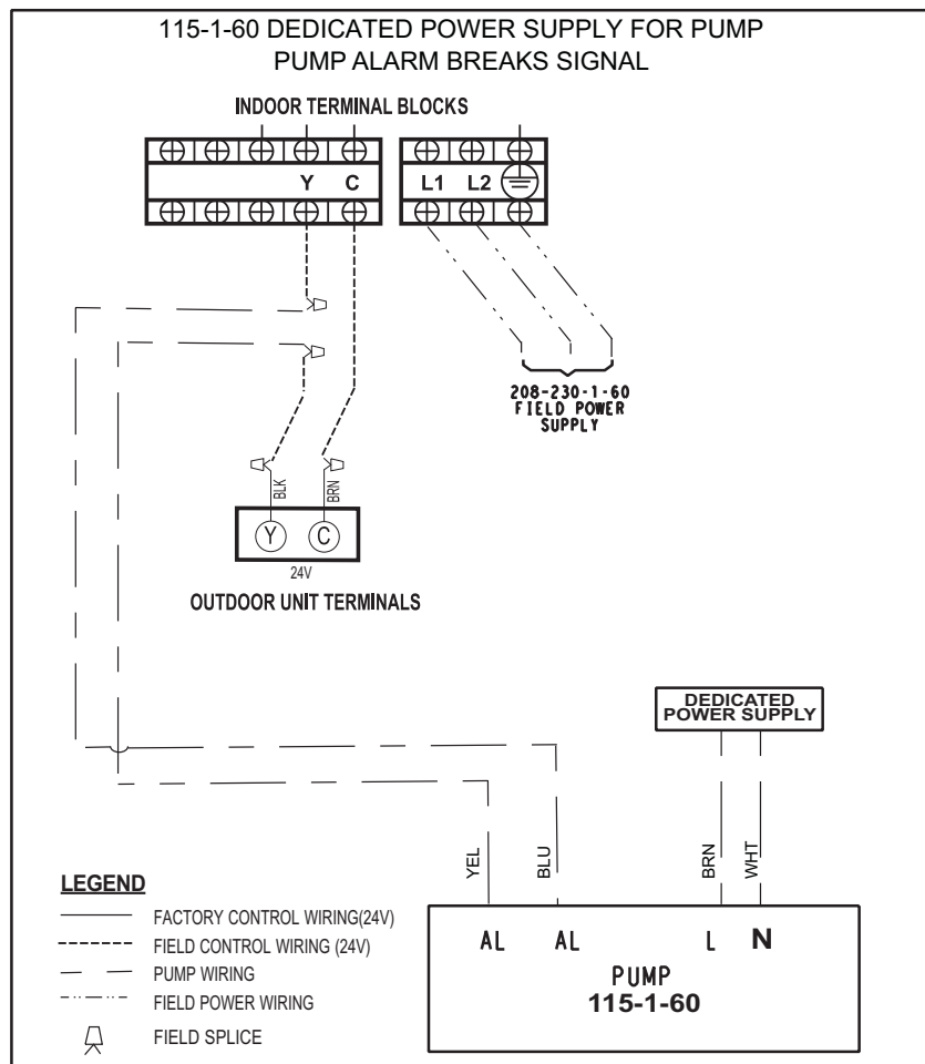
Fig. 25 – Installing a 115-1-60 Pump in a 208-230-1-60 40MK*F Under Ceiling AC Unit
