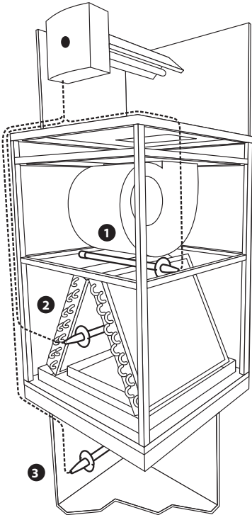
Mounting Options
