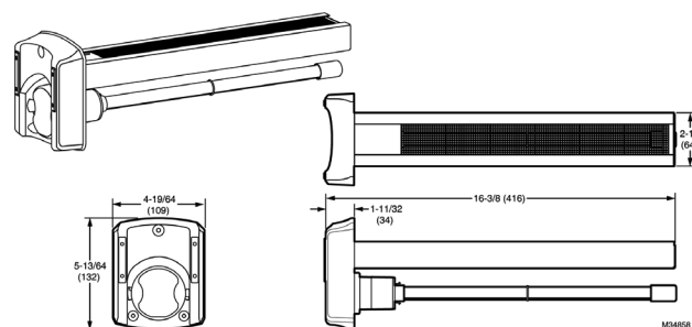
Fig. 1. UV2400U5000, dimensions in inches (mm).
