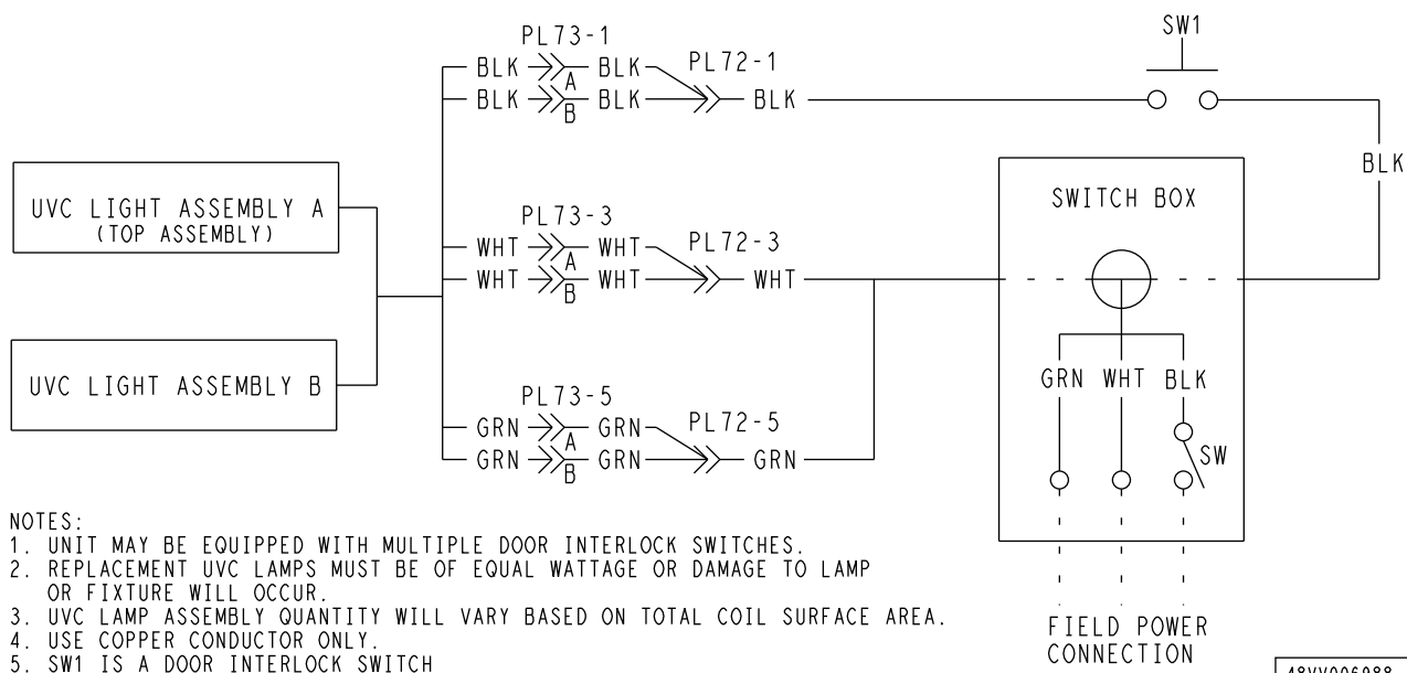
Fig. 7 — 48/50V UV-C Section Wiring Diagram
