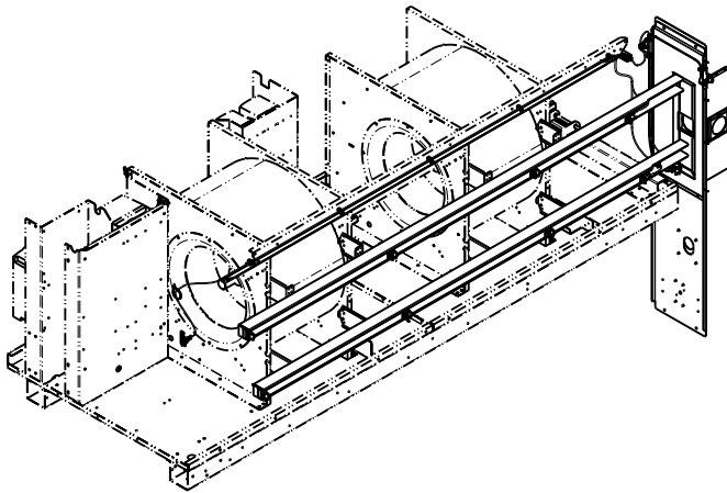
Fig. 3 — Typical UV-C Lamp and Fixture Kit Installation on 48/50K 20-60 Tons
