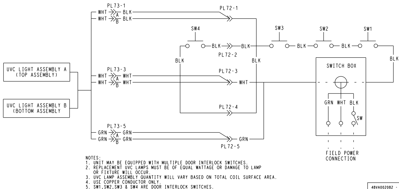
Fig. 6 — 48/50K UV-C Section Wiring Diagram
