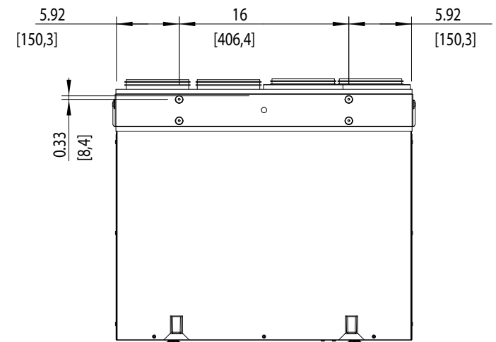
(Wall Bracket) Hanging Hole Pattern Back View
