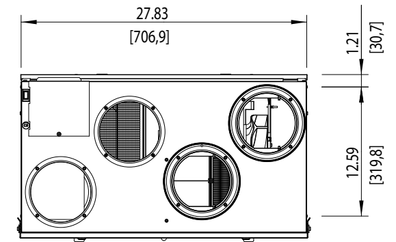
(Ceiling Chain) Hanging Hole Pattern Top View
