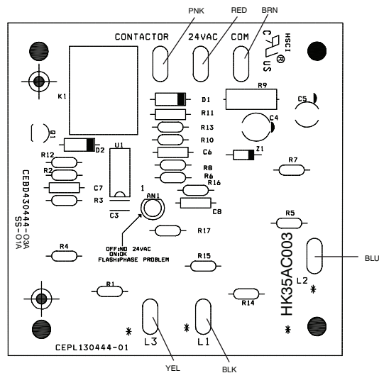
Fig. 4 - Phase Monitor Module Detail (208/230V and 460V)
