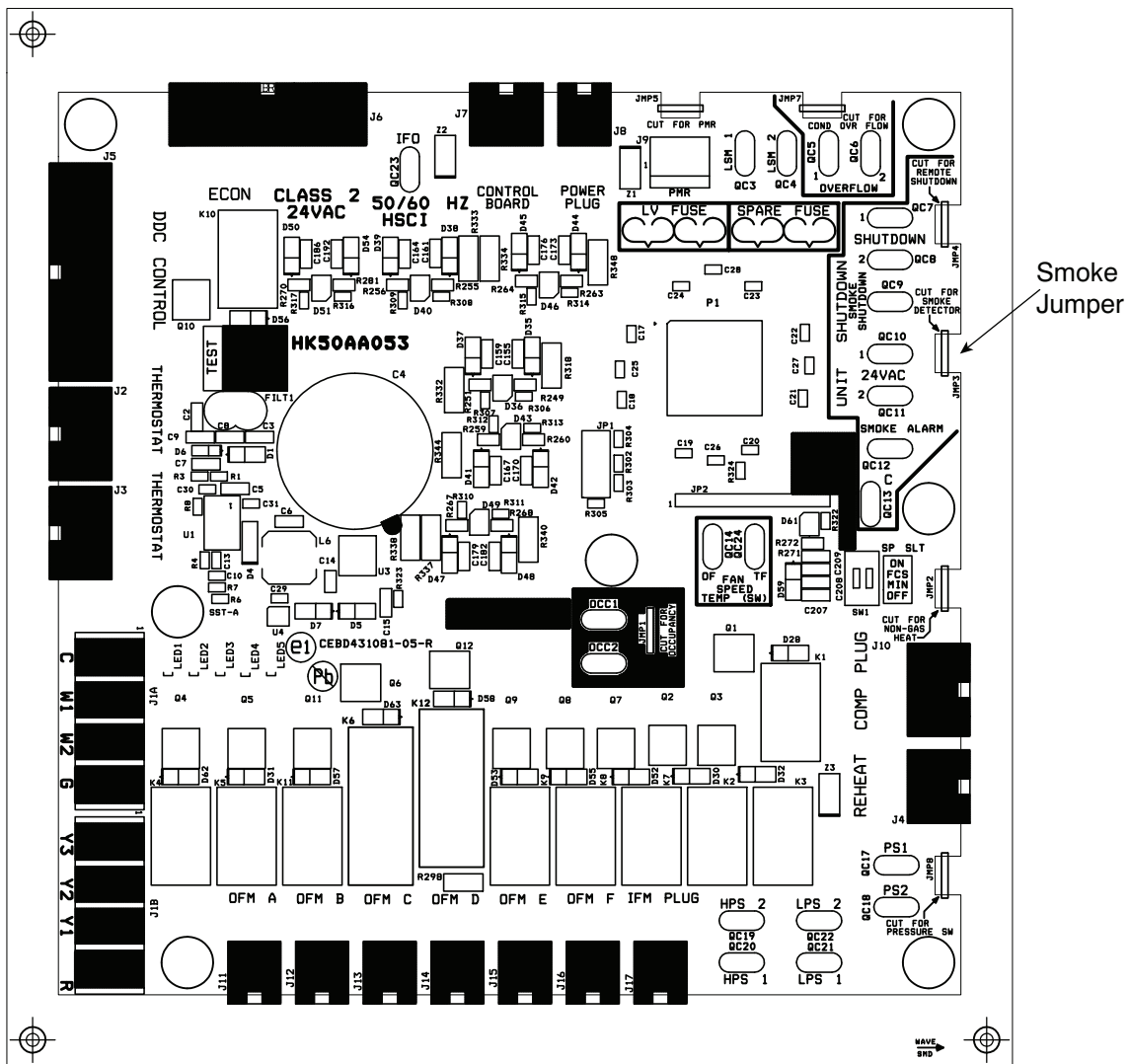
Fig. 3 - 48/50LC Control Board
