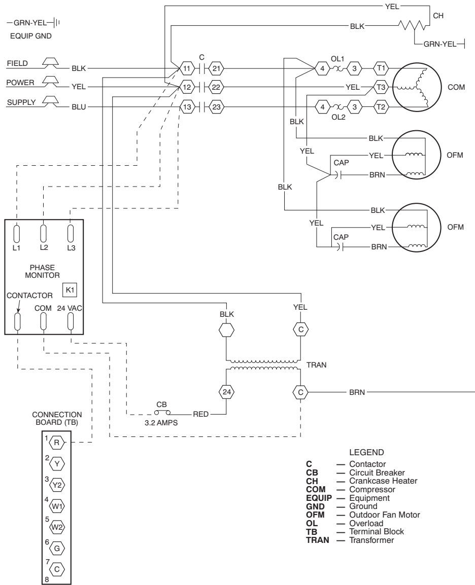
Fig. 1 - Typical Wiring Phase Monitor
