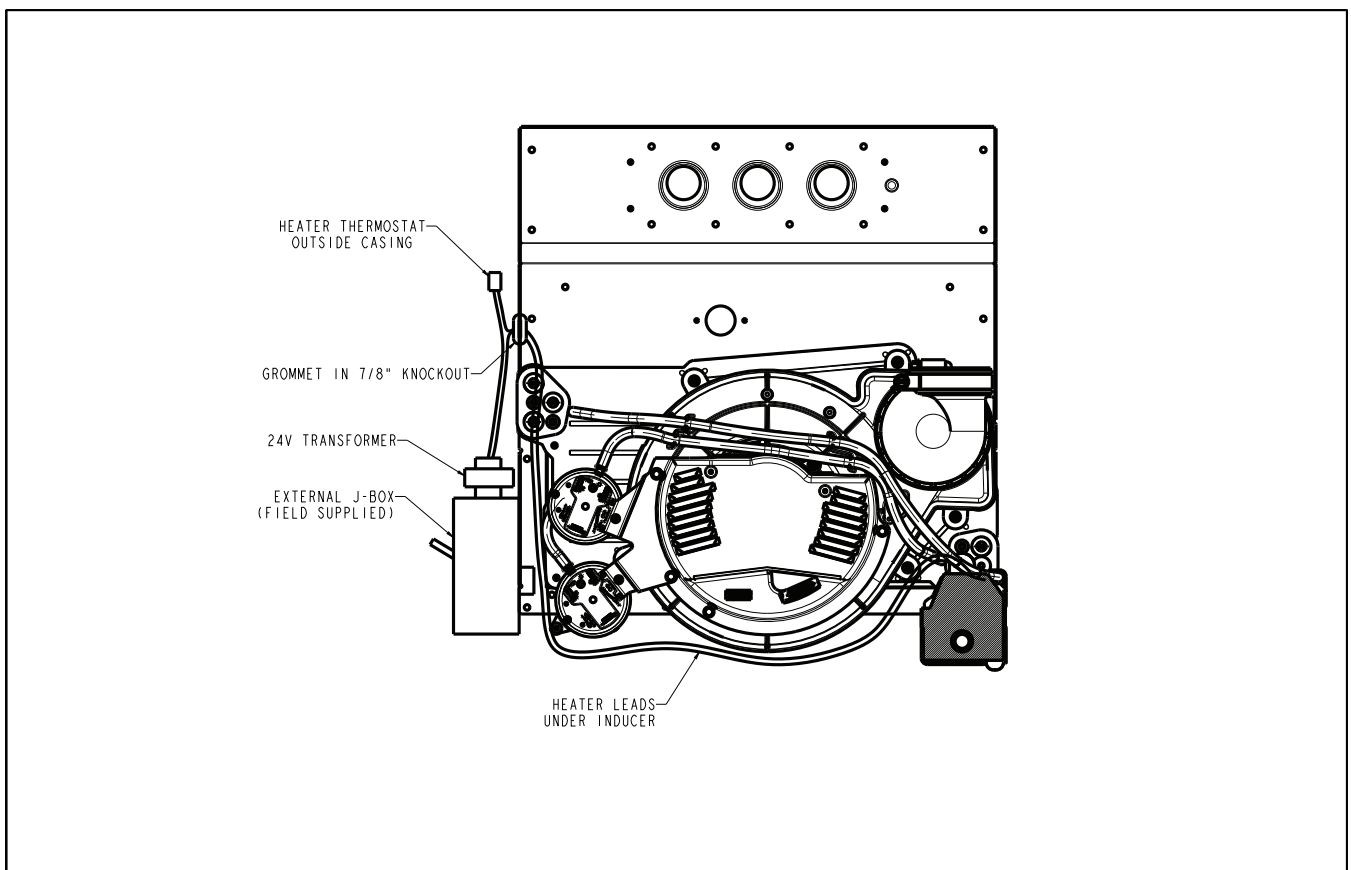
Fig. 2 - Wire Routing
