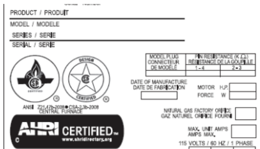
Fig. 4 – Rating Plate
