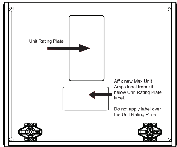
Fig. 5 – Max Unit Amps Label Location
