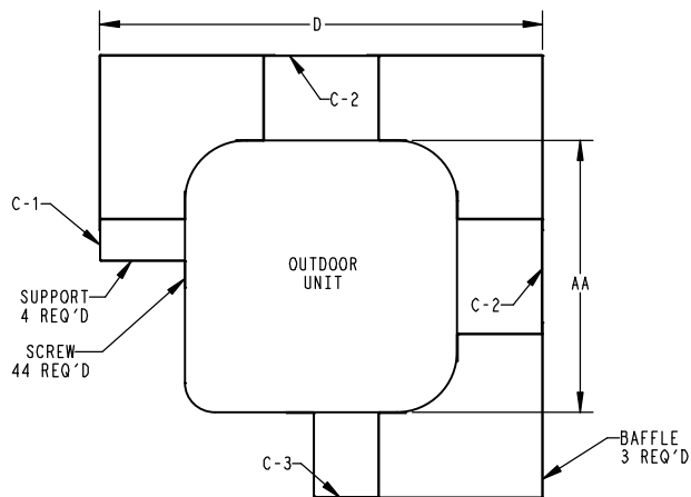
BAFFLE ASSEMBLY
