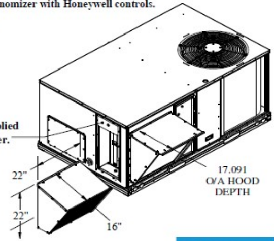
Direct coupled actuator mount
