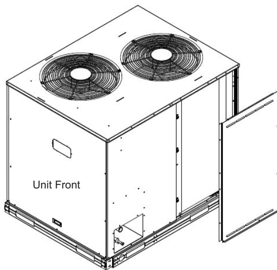
Fig. 2 — Typical Third Panel Hail Guard Installation (Uses 8 Grommets, 4 on Each of 2 Corner Posts)
