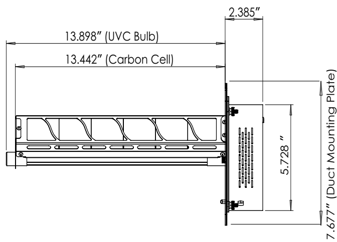
Fig. 1 – Dimensions (in.)
