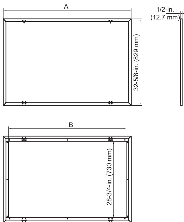
Fig. 1 - Access Panel Dimensions
