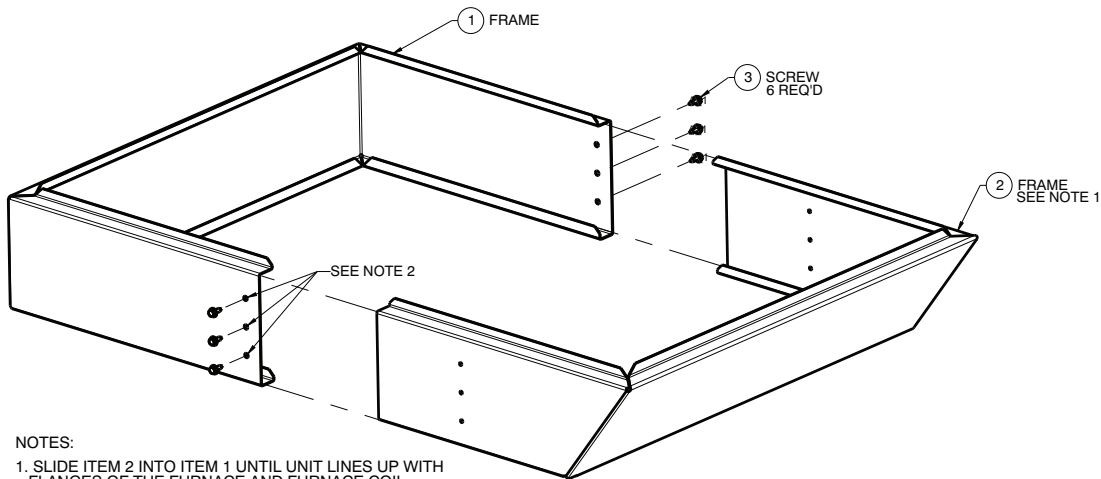
Fig. 1 - Coil Adapter - Coil Width Same as Furnace
