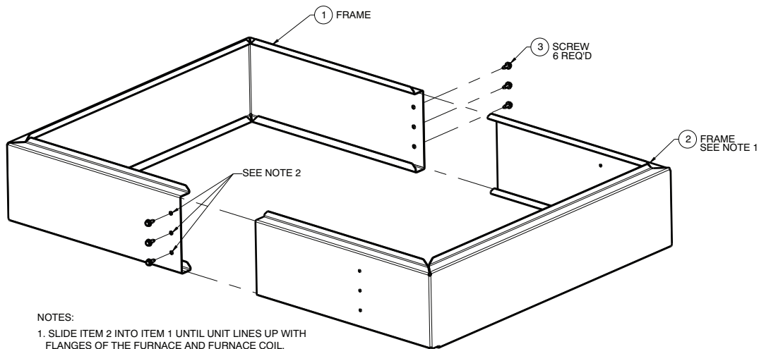
Fig. 1 - Coil Adapter - Coil Width Same as Furnace
