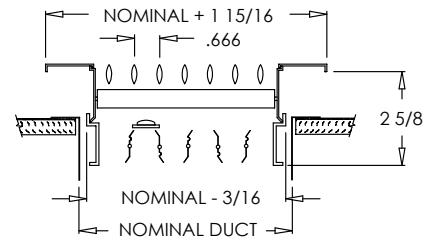
933-O (Stamped Steel One Piece Frame)
