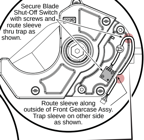
Right Side-Front Gearcase Assembly
