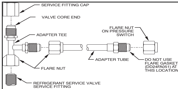
Fig. 1 - High-Pressure Switch Refrigerant Connections for Air Conditioners
