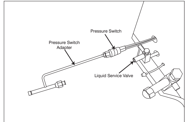
Fig. 2 - High-Pressure Switch Adapter Connections
