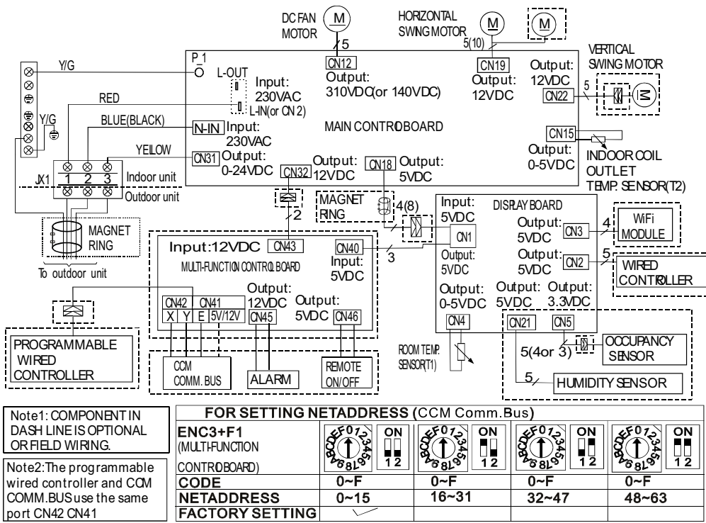
Fig. 13 —Wiring Diagram - Size 18K
