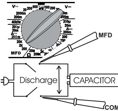
Capacitance (MFD)
