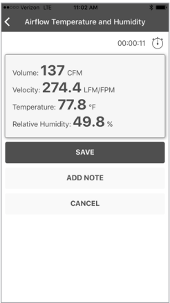
Airflow Temperature and Humidity test data
