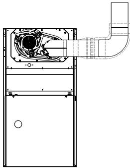
Upflow Application-Vent Elbow Up
