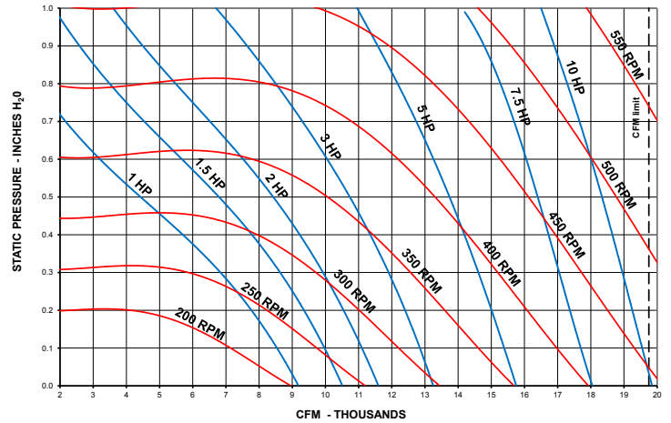
ID/IS/IUP800 w/ WS844 - Airflow Data
