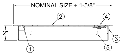
SECTION VIEW
