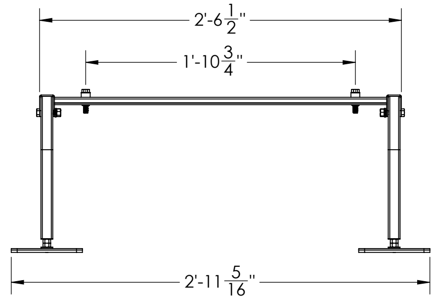
END VIEW RETRACTED
